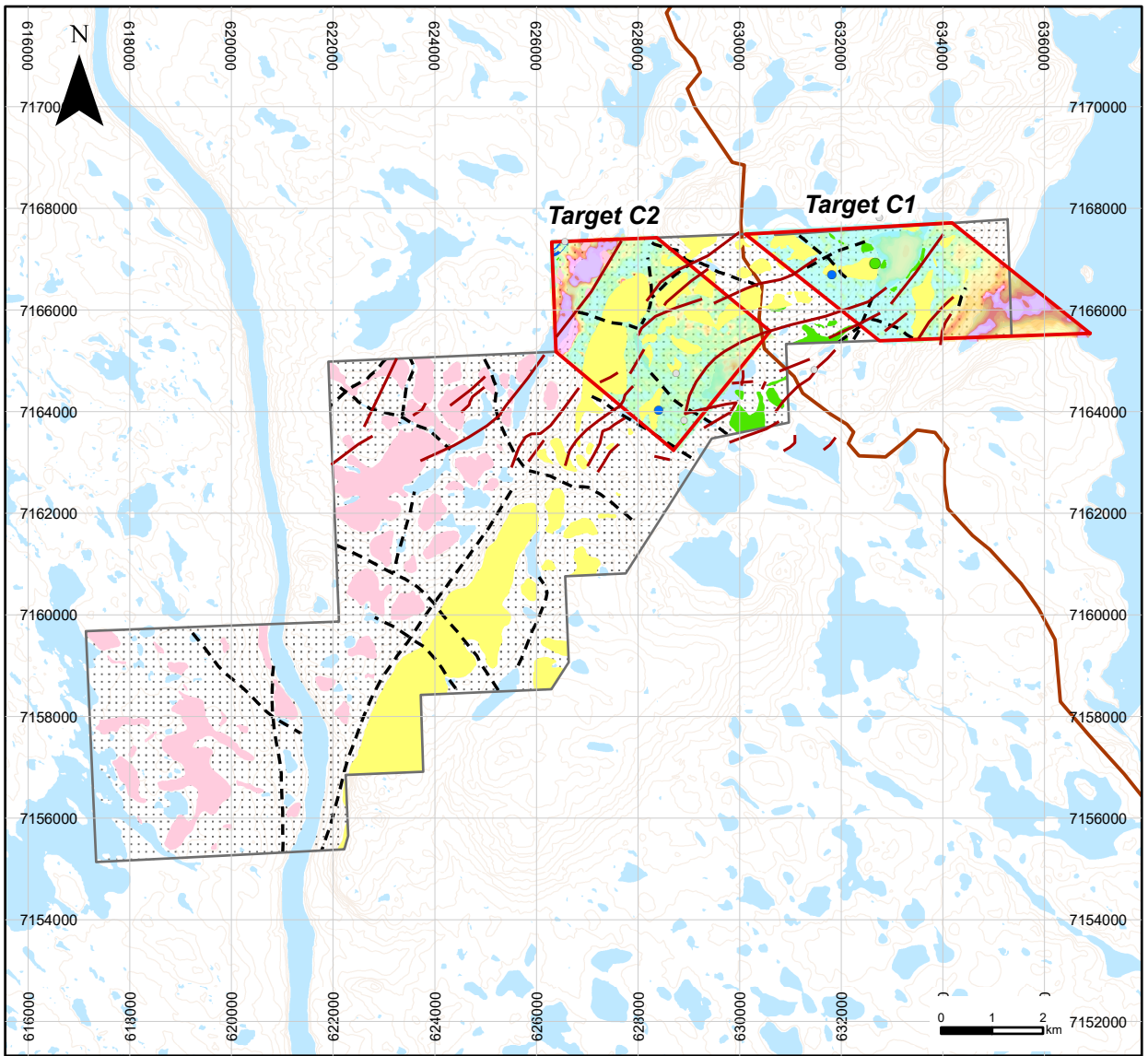
Block C – Target C1 – VTEM Results with Geology
